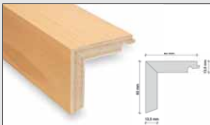
Stair nosing with connection on one side
