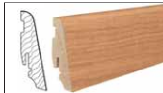
Stick-on skirtings with solid wood core, veneered, oiled, 19 x 58 mm
