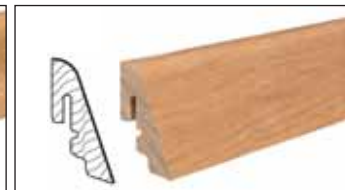
Stick-on skirtings with solid wood core, veneered, matt finished, 19x39 mm
